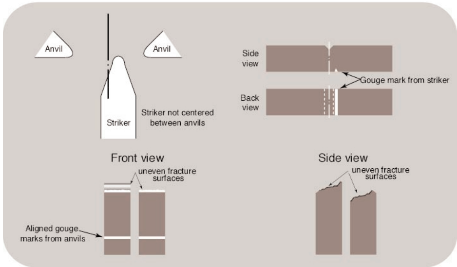
Figure 3. Off-Center Striker.
